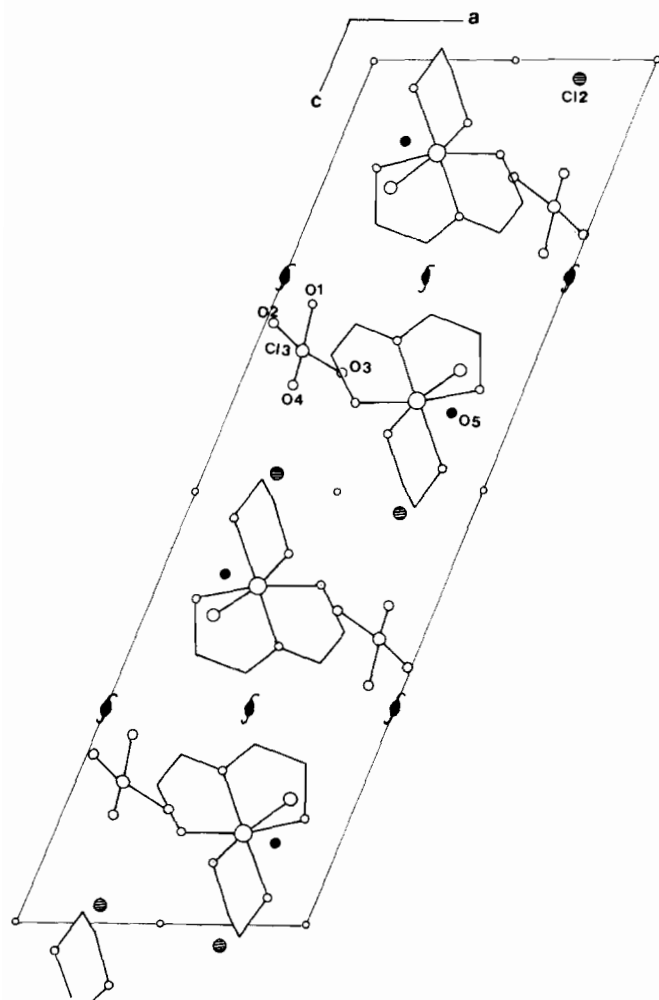
Fig. 2. The packing diagram for [\text{Co}(\text{en})\{\text{NH}_2(\text{CH}_2)_2\text{N}=\text{CHCH}_2\text{NH}_2\}\text{Cl}]\text{Cl}(\text{ClO}_4)\cdot\text{H}_2\text{O} viewed along the b-axis and the atom numbering scheme for \text{ClO}_4^- , \text{Cl}^- , and O in \text{H}_2\text{O} .
